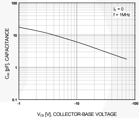
Figure 4. Output Capacitance
